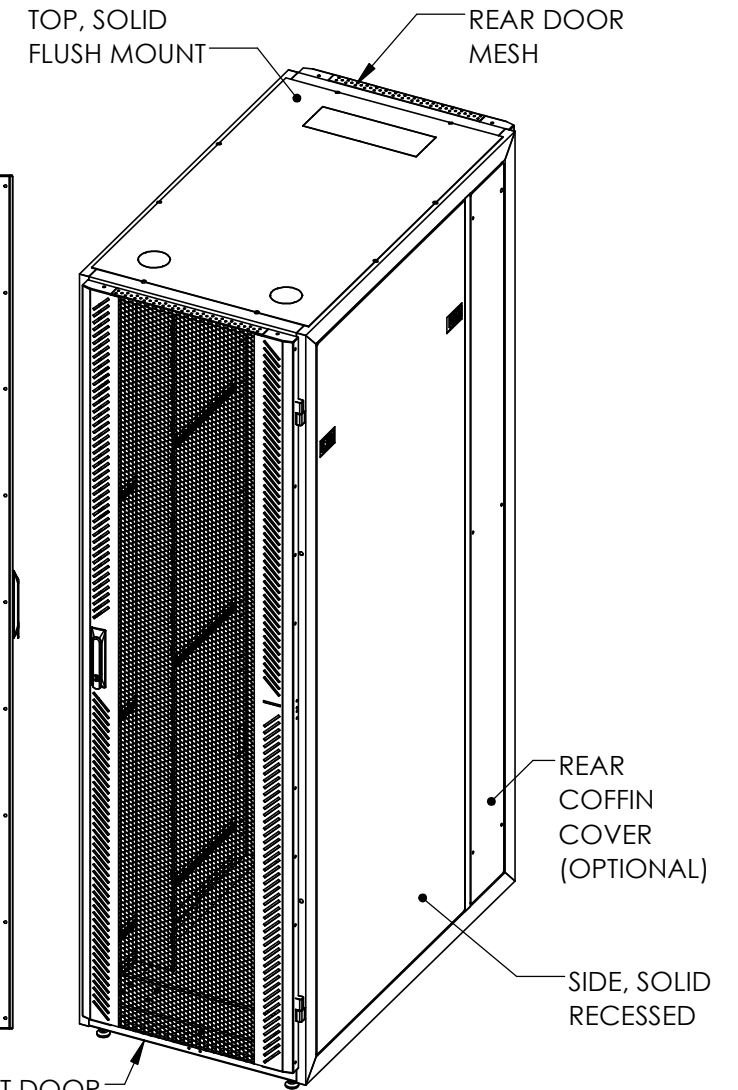
ISOMETRIC VIEW
