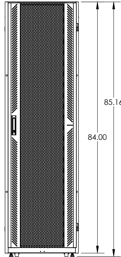
FRONT VIEW
