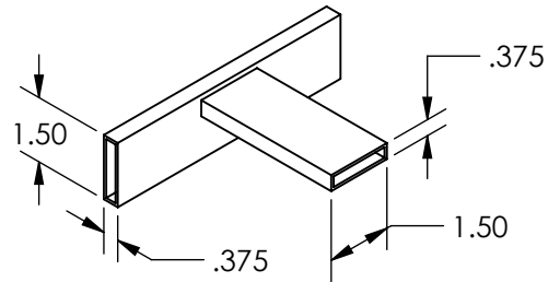
STANDARD RUNWAY ISOMETRIC SECTION VIEW
